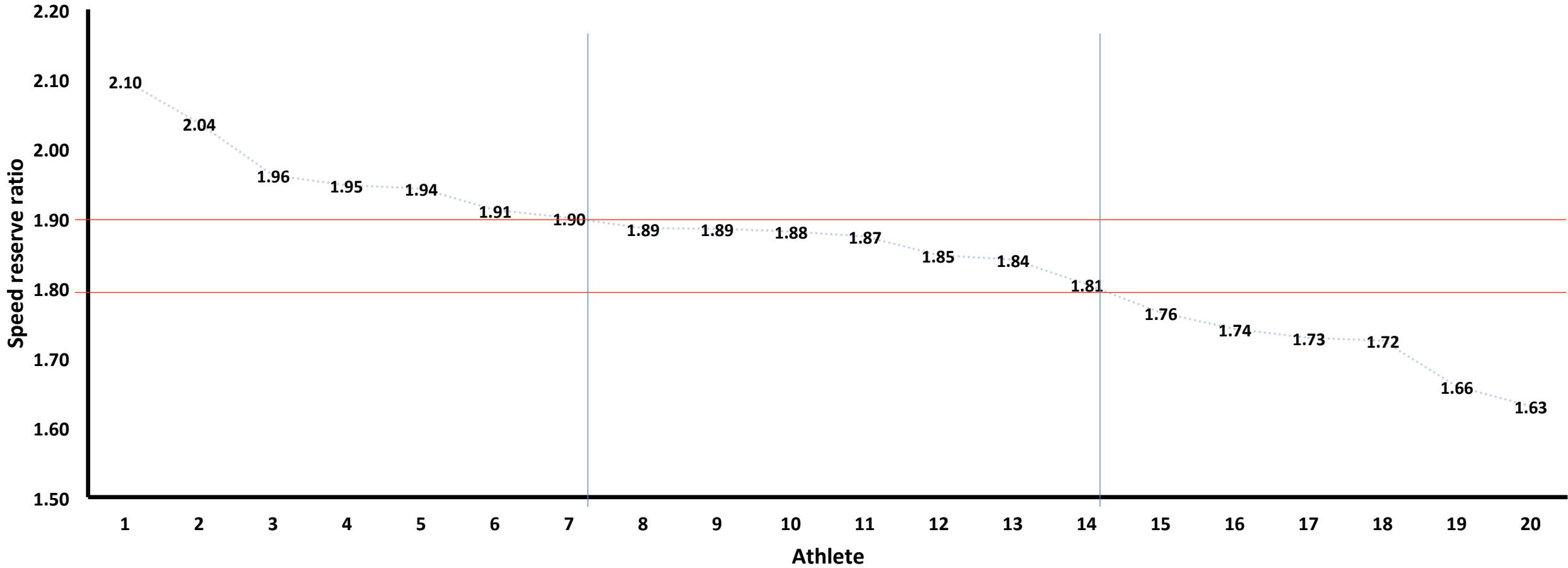
Speed Reserve Ratio (SRR) of England Cricket Athlete Profiles
